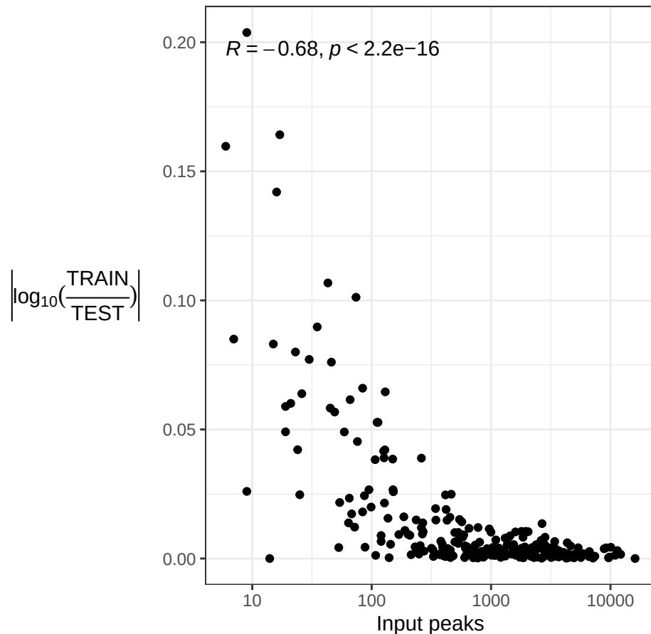
TRAIN/TEST RATIO vs N.PEAKS
