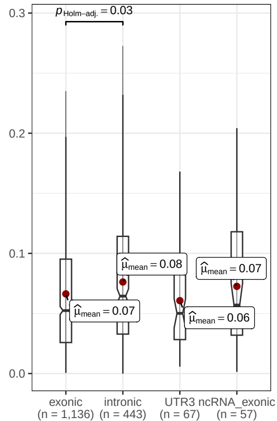
KDM-5 (Inf)
