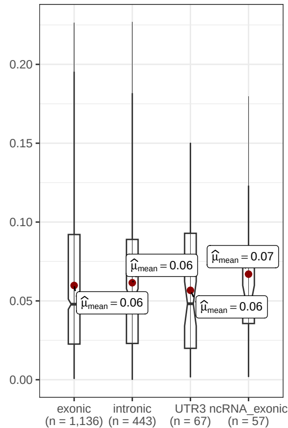
KDM-3 (Inf)
