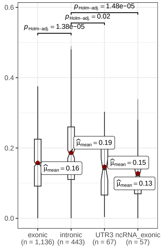
KDM-2 (Inf)
