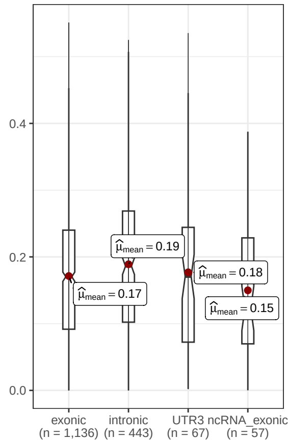
KDM-1 (Inf)
