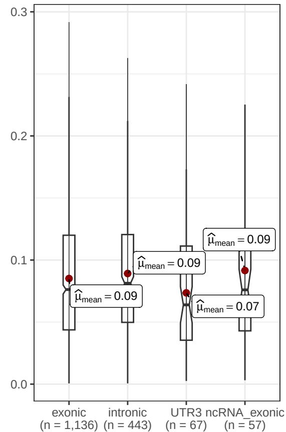
KDM-4 (Inf)
