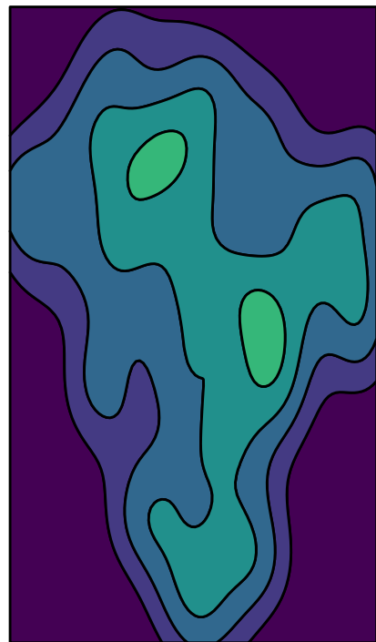
exonic
