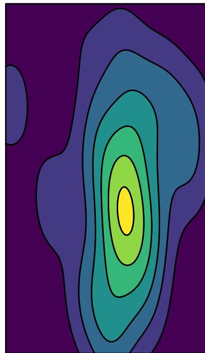
ncRNA_exonic
