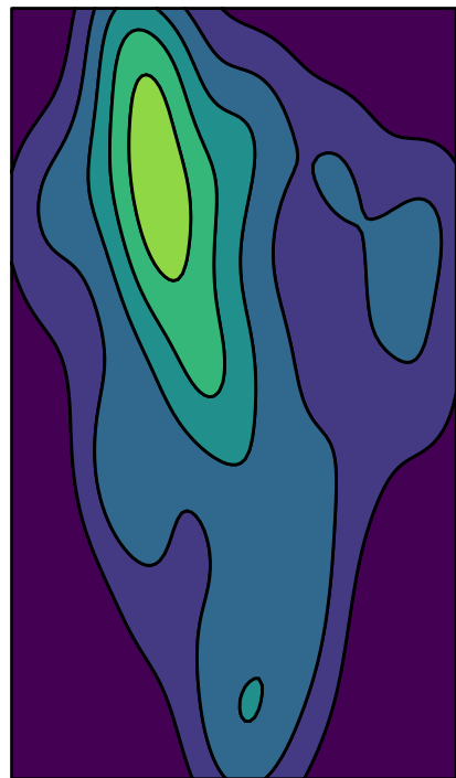
intronic
