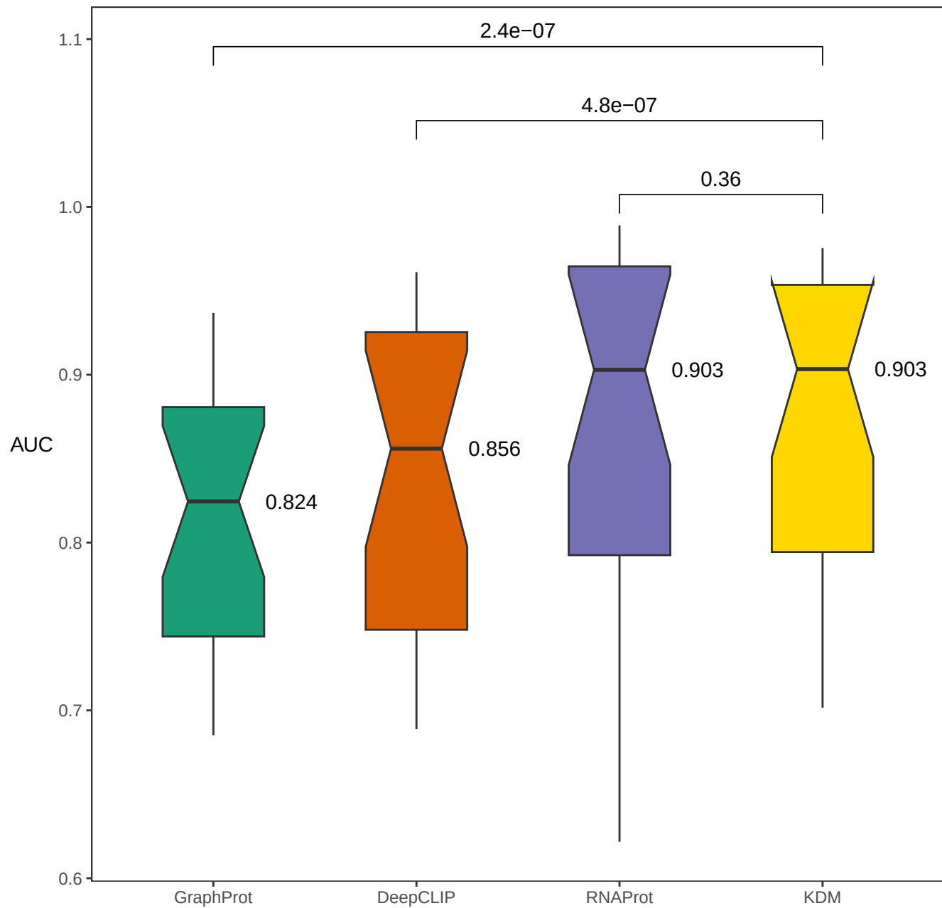
AUCs on RBP_24 with RNAProt datasets
