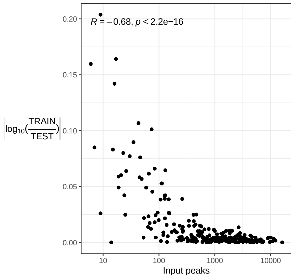
TRAIN/TEST RATIO vs N.PEAKS
