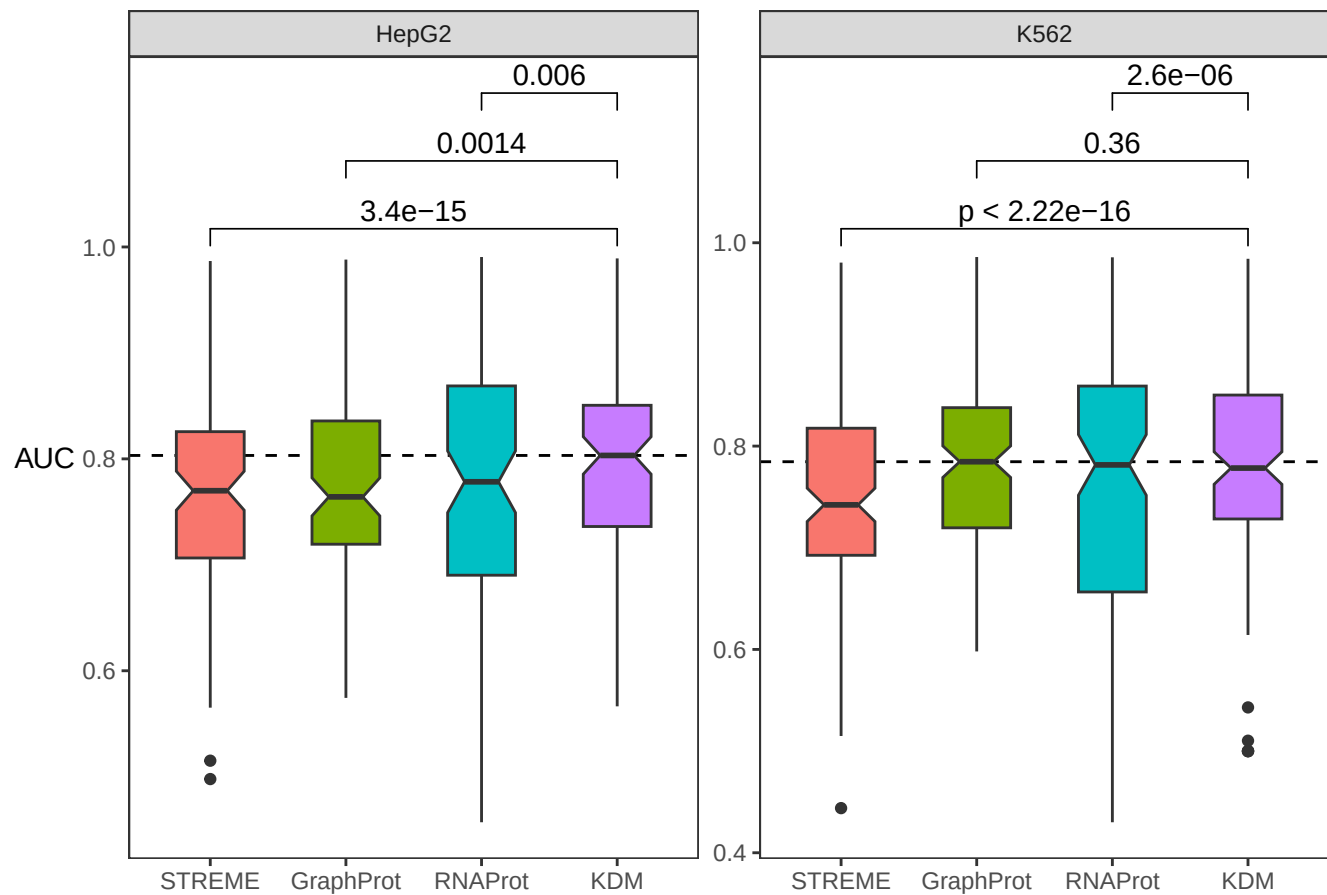
AUC distributions ~ Cell.line
