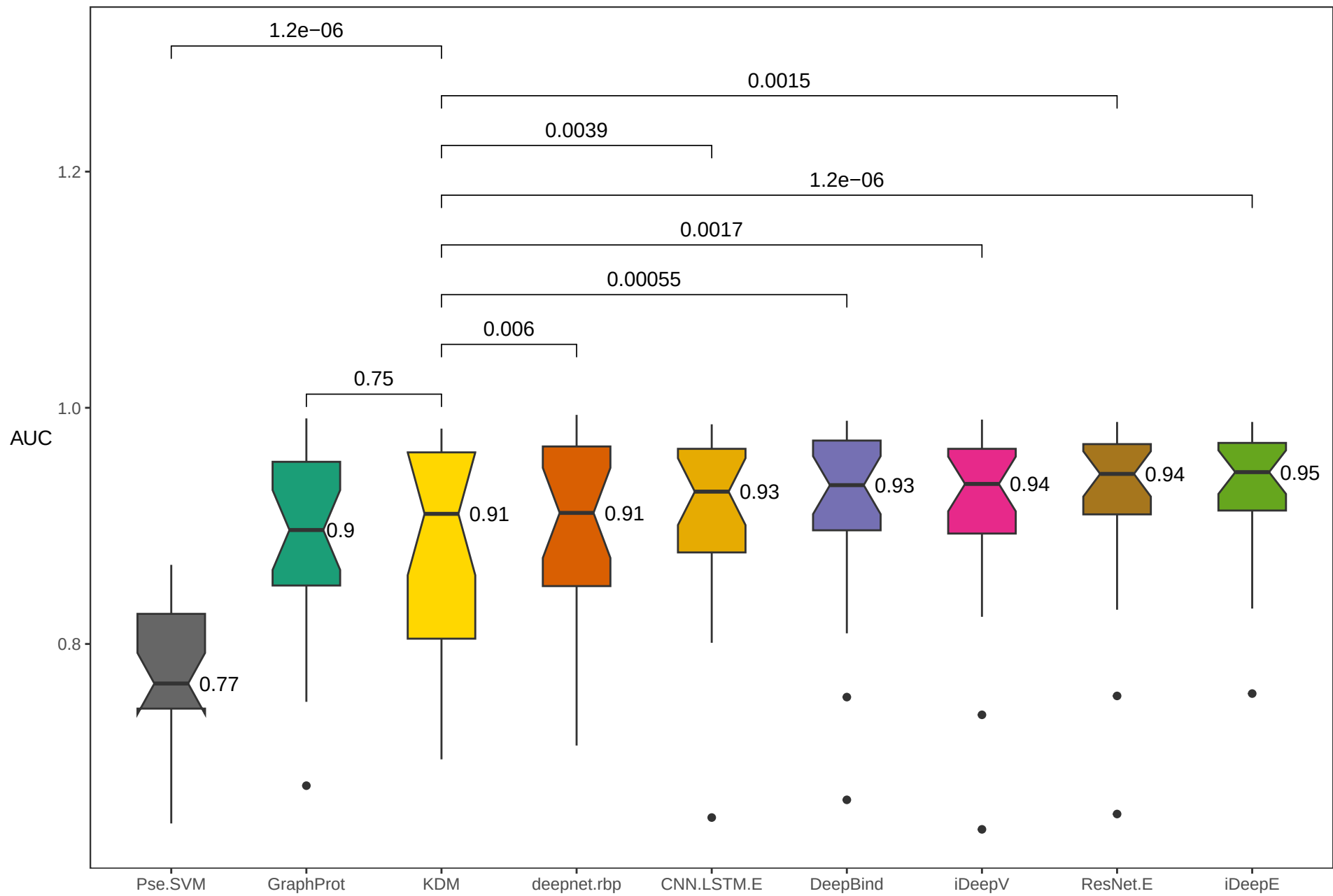
AUCs on RBP_24 with GraphProt datasets
