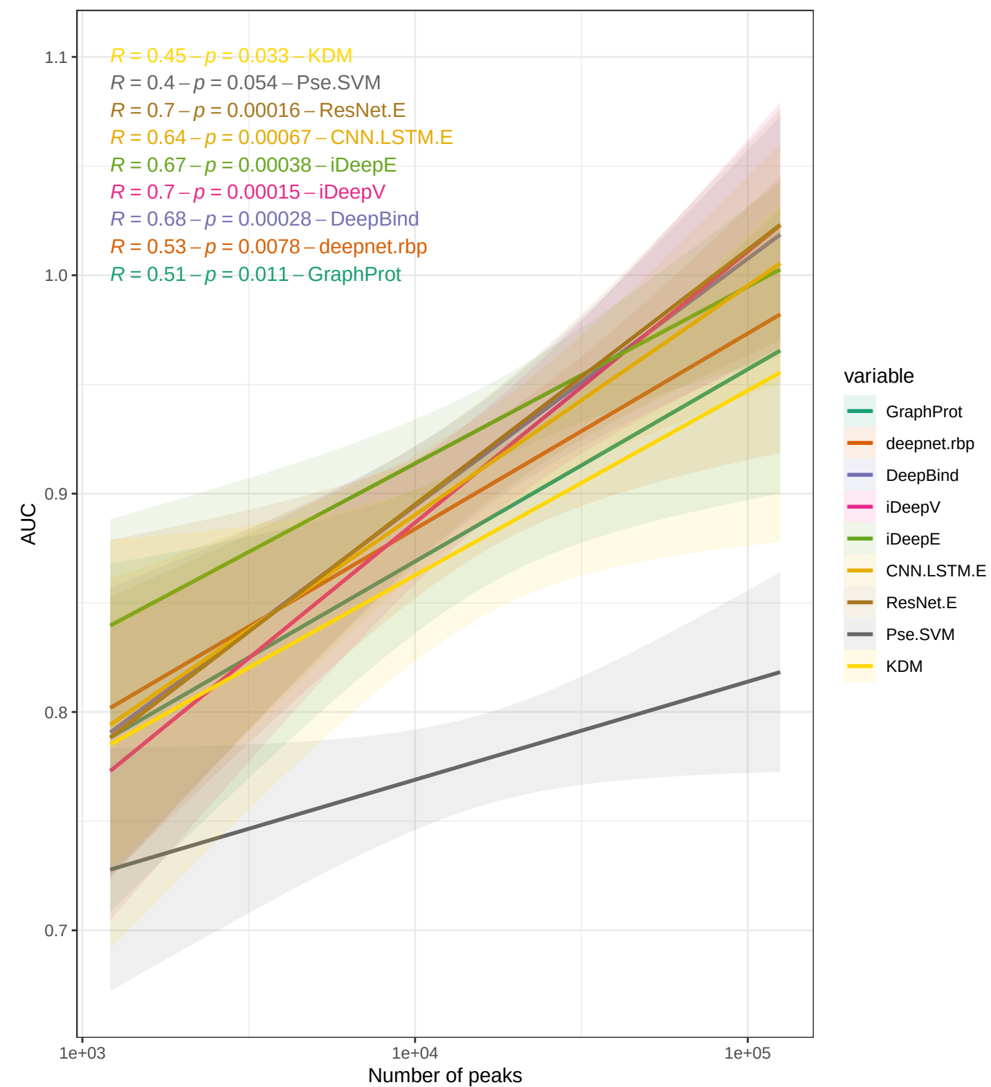
AUC ~ log10(N.Peaks)
