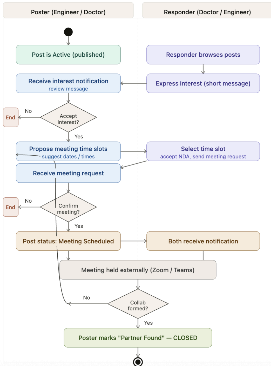
Activity Diagram 3 — Meeting Request Workflow
