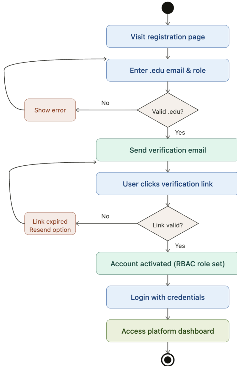
Activity Diagram 1 — User Registration &amp; Login
