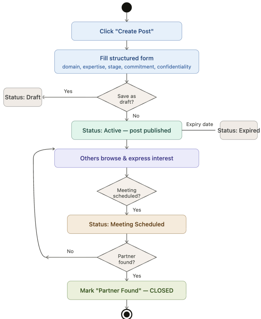
Activity Diagram 2 — Post Creation &amp; Lifecycle
