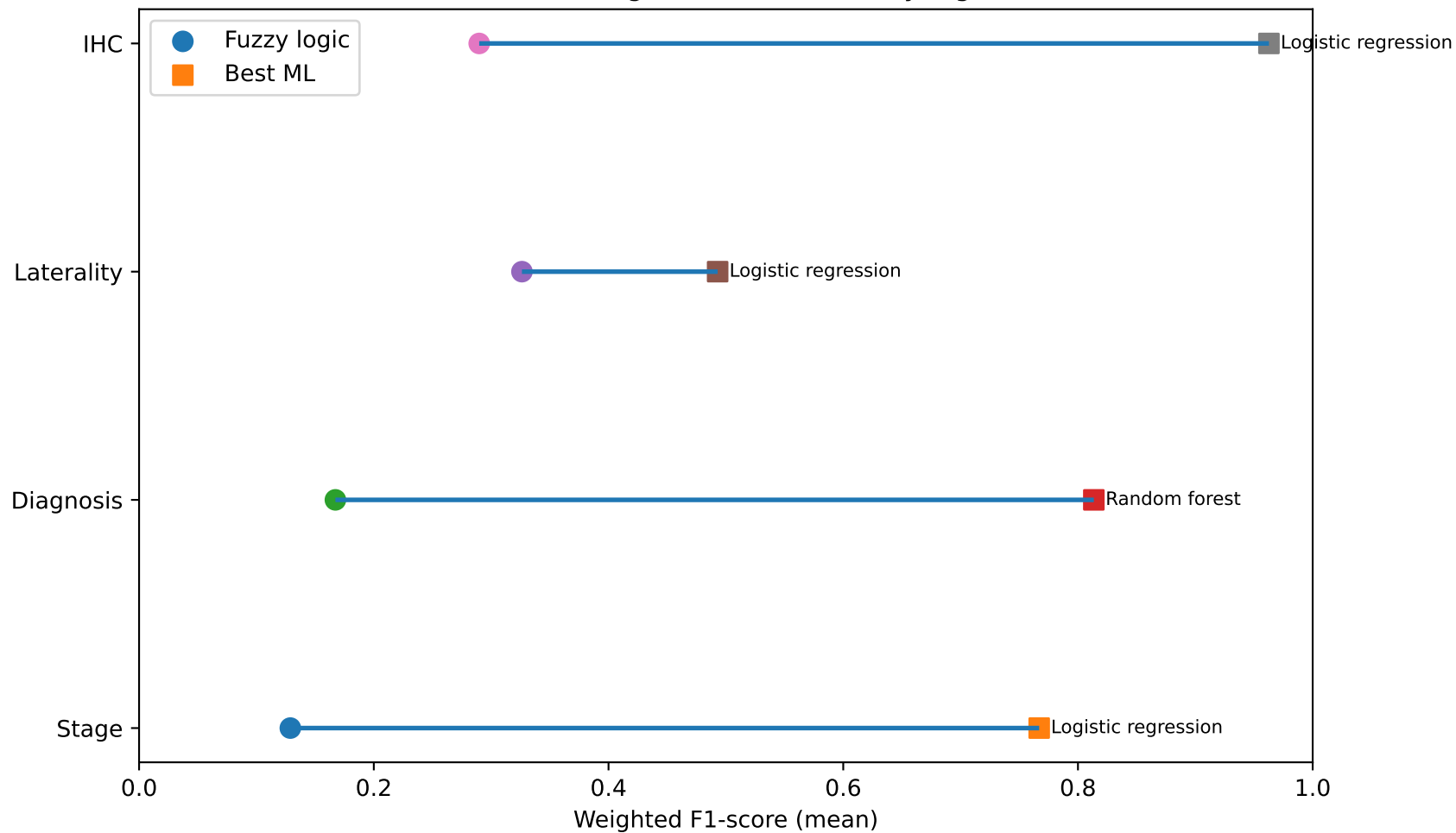
Best machine-learning model versus fuzzy-logic baseline
