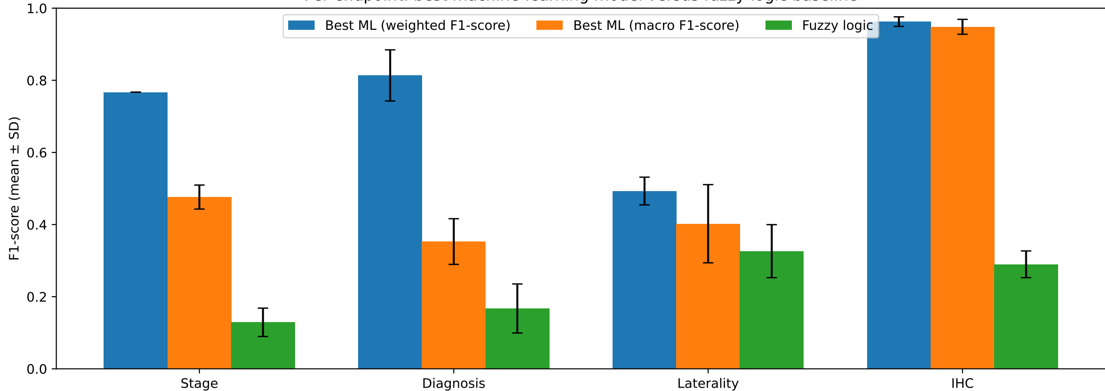
Per endpoint: best machine-learning model versus fuzzy-logic baseline
