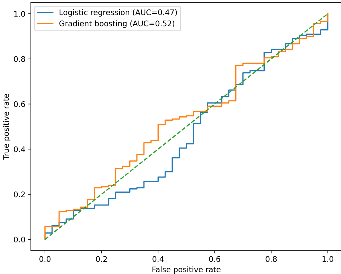
Stage classification ROC curves for top ML models
