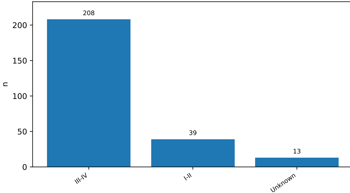
Stage
