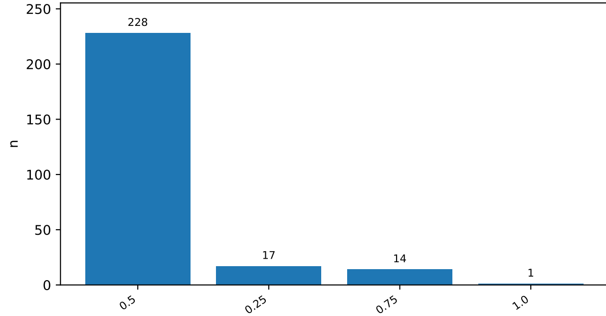
Diagnosis
