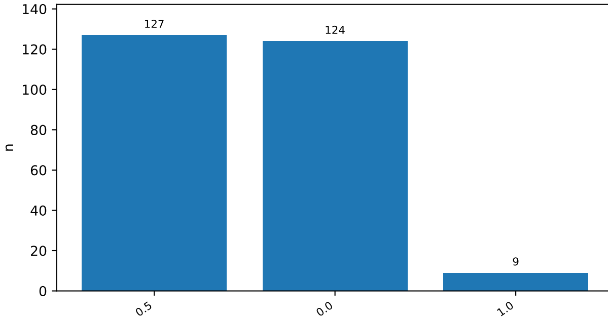
Laterality
