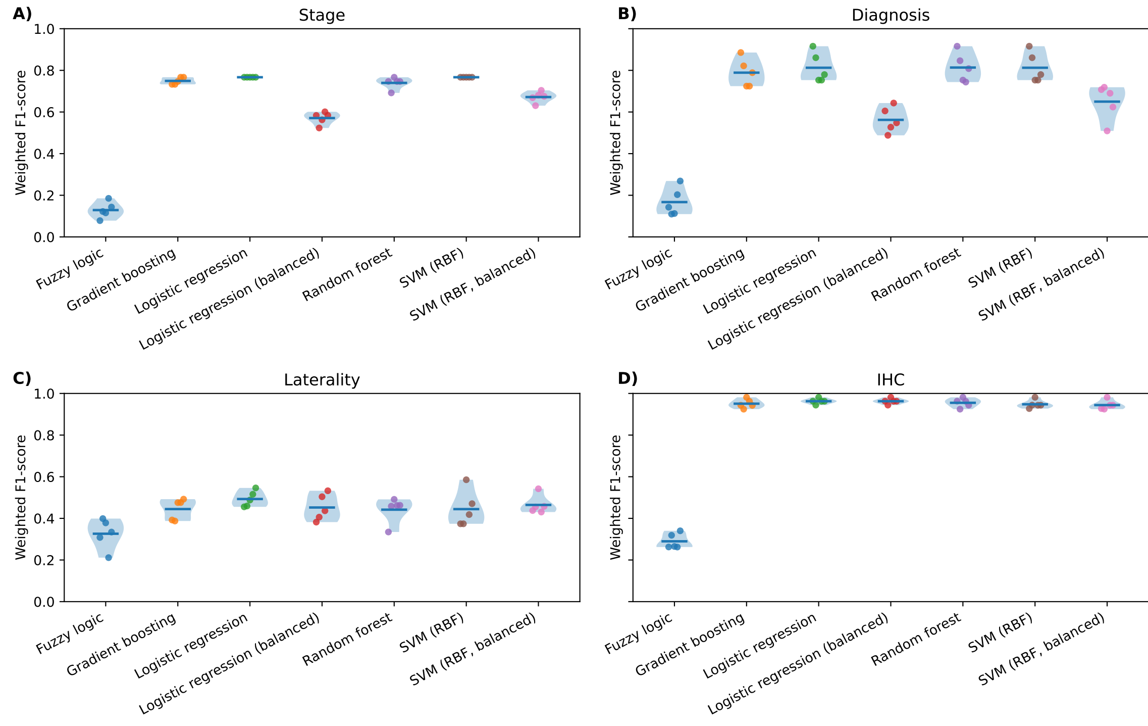
Fold/seed-wise weighted F1-score distributions across repeated splits
