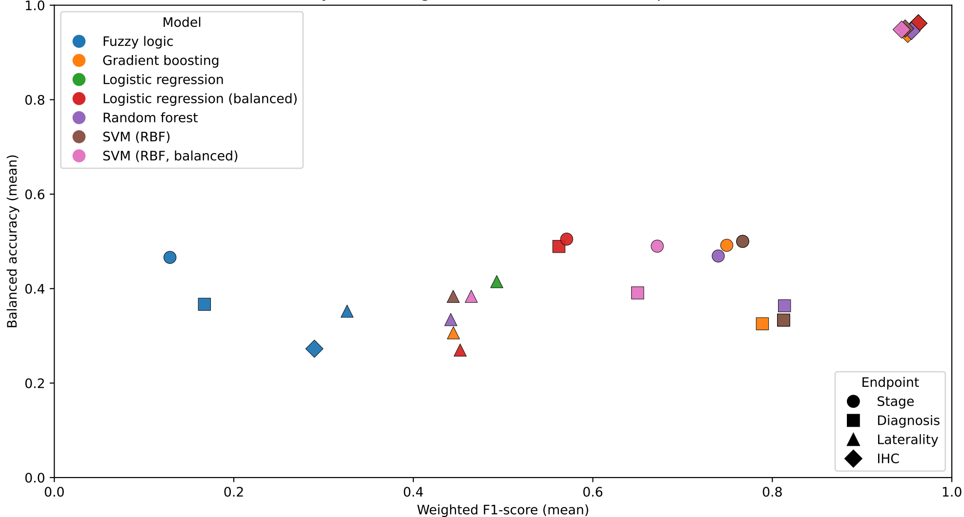
Balanced accuracy versus Weighted F1-score (marker = endpoint; color = model)
