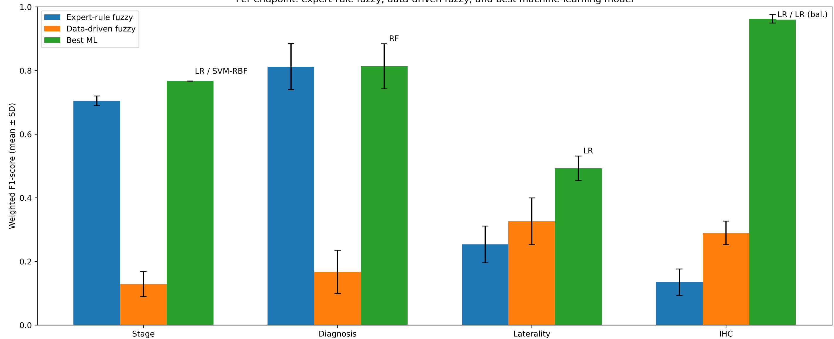
Per endpoint: expert-rule fuzzy, data-driven fuzzy, and best machine-learning model
