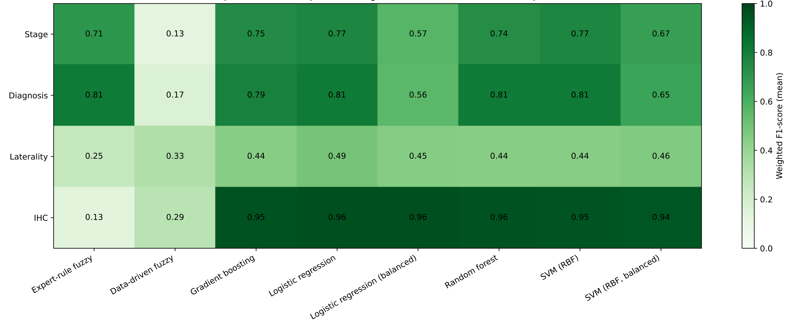
Model performance comparison (Weighted F1-score; mean across 5 repeats)
