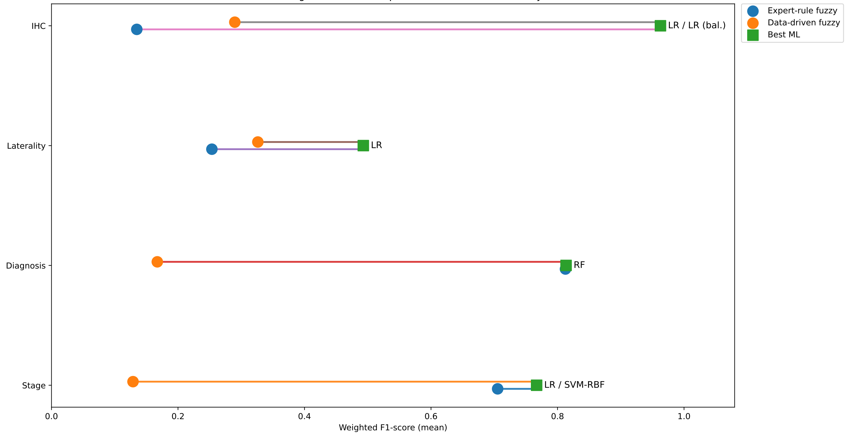
Best machine-learning model versus expert-rule and data-driven fuzzy baselines
