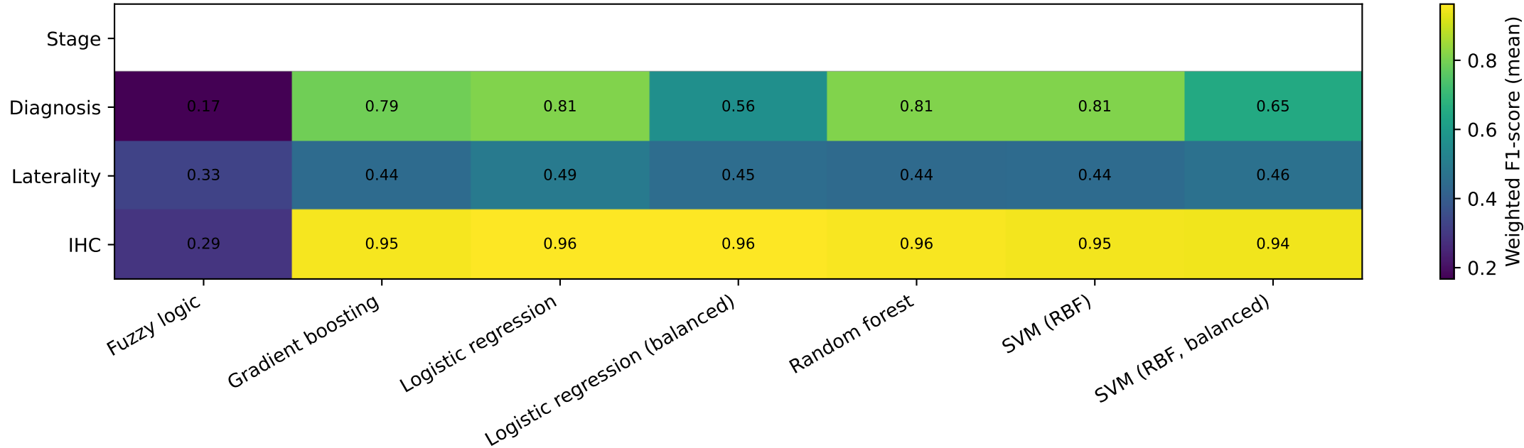
Model performance comparison (Weighted F1-score; mean across 5 repeats)
