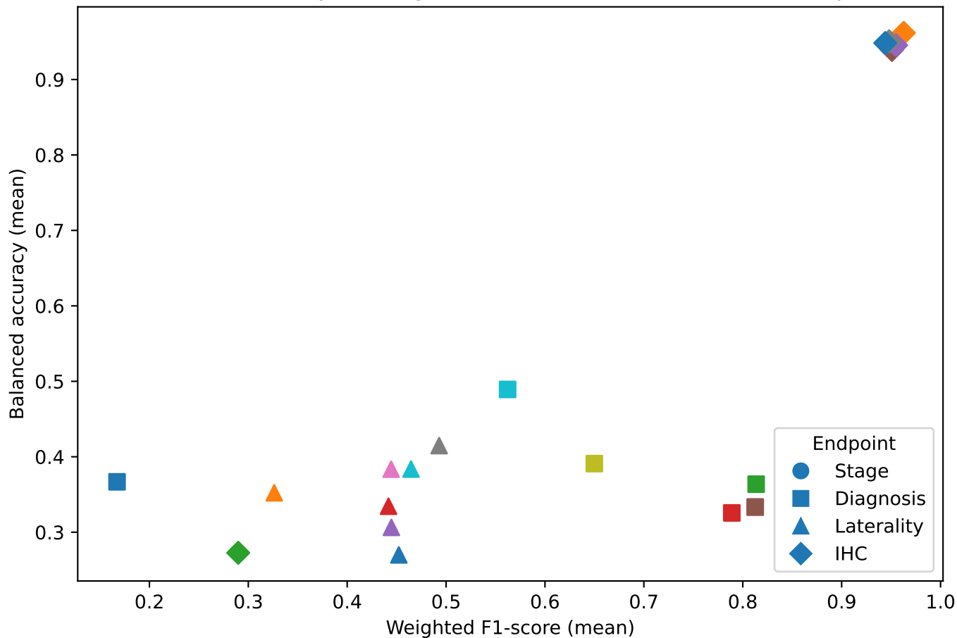
Balanced accuracy vs Weighted F1-score (marker indicates endpoint)
