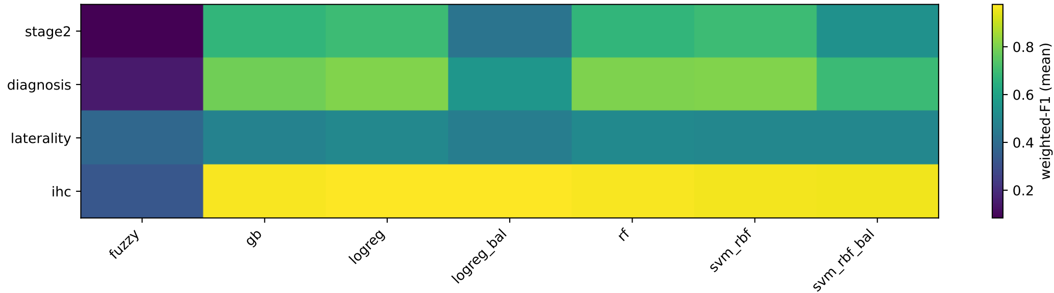
Model comparison (weighted-F1 mean) — repeated stratified 80/20
