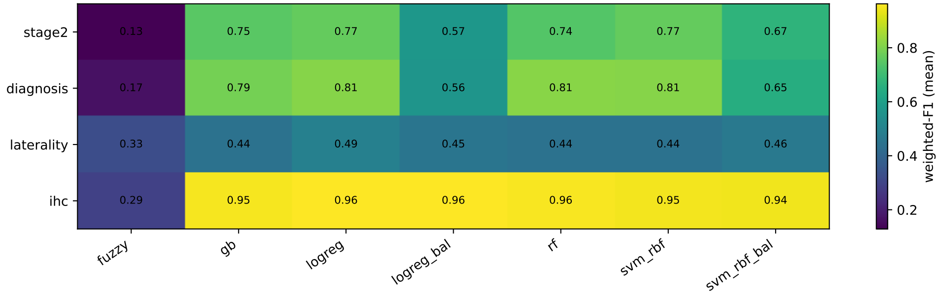
Model comparison (weighted-F1 mean \pm across 5 repeats; stratified 80/20)
