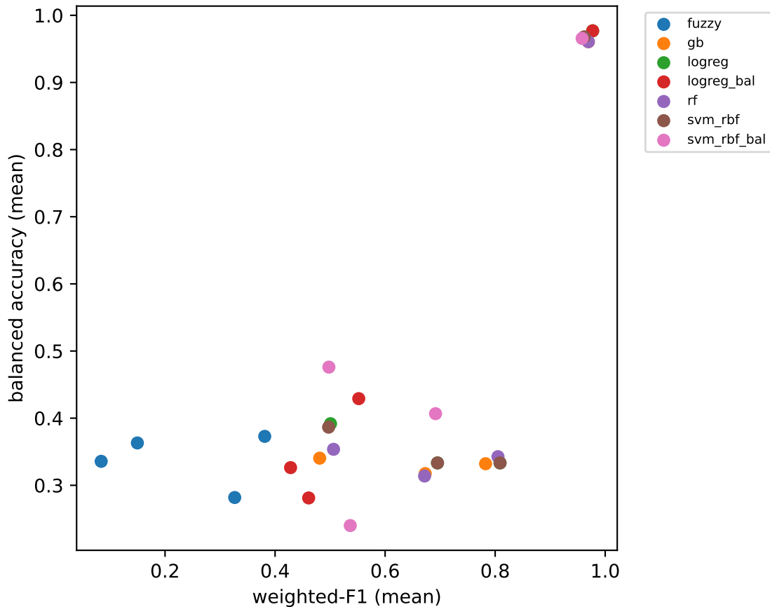
Imbalance-aware view: balanced acc vs weighted-F1
