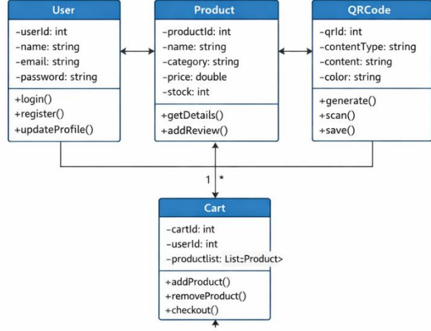
QR E-Ticaret Class Diagram
