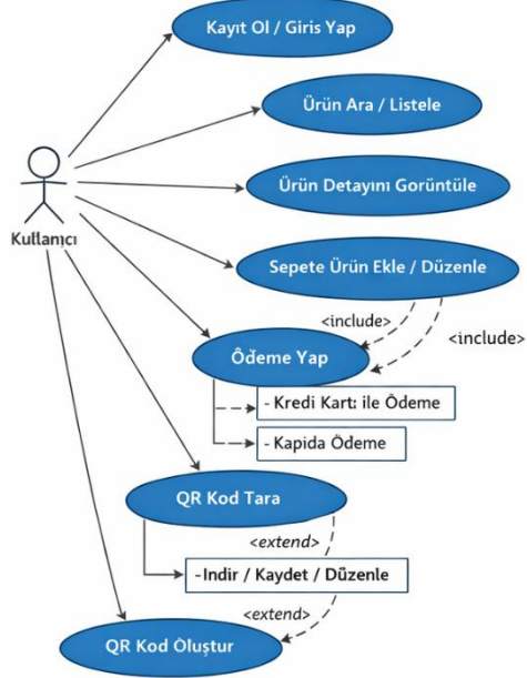
QR E-Ticaret Use Case Diagram
