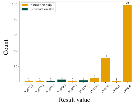
Figure 8: Distribution of result values in \mu -instruction skip test (successful glitches only)
