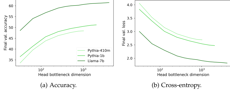
Figure 1.4: Effect of reducing the LM Head rank on accuracy and cross-entropy. Figures from Godey, Clergerie, and Sagot [46].
