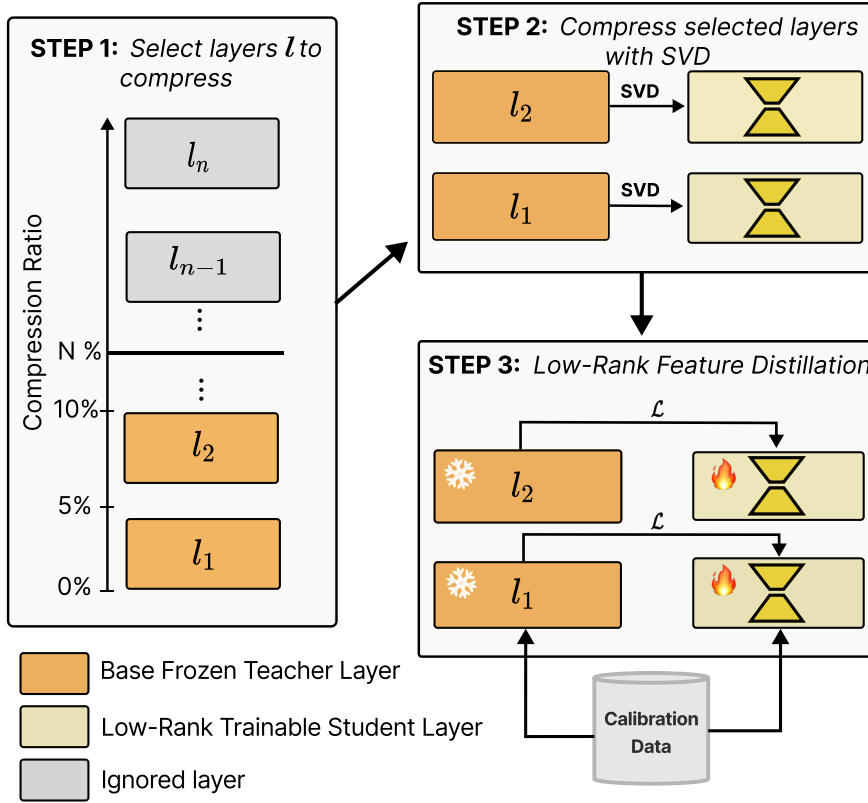
Figure 3.1: Lillama approach : STEP 1 selects layers to compress for a target compression ratio (e.g., N\% ) using various strategies (see Section 3.6). STEP 2 compresses and initializes the chosen parameters via SVD. STEP 3 distills the low-rank weights with a small calibration dataset.
