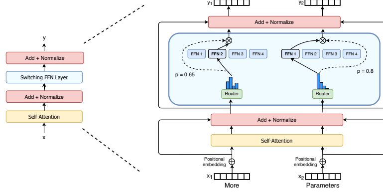
Figure 2.8: Switch Transformer encoder block, where the dense feed-forward layer is replaced by a sparse Switch FFN layer. Figure adapted from Fedus, Zoph, and Shazeer [40].
