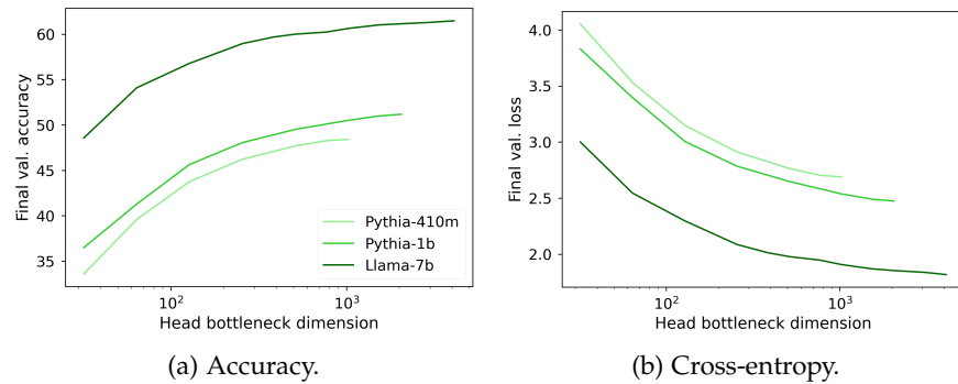
Figure 1.3: Effect of reducing the LM Head rank on accuracy and cross-entropy. Figures from Godey, Clergerie, and Sagot [52].
