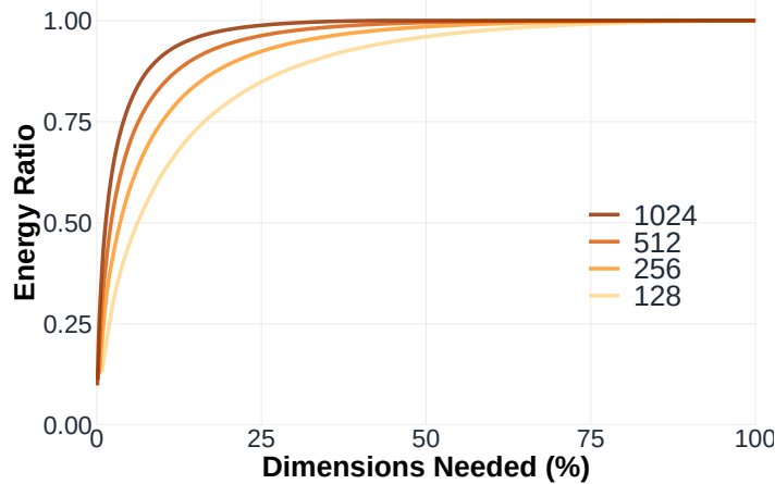
Figure 5.5: Dimensions needed for a given energy ratio.
