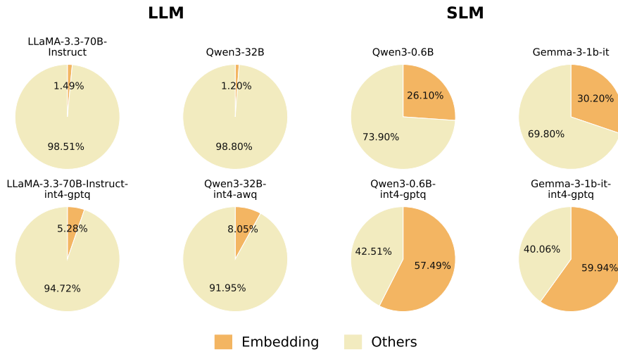
Figure 1.2: Proportion of the size in MB of embedding parameters across different model sizes. Data taken from https://blog.squeezebits.com/vocabulary-trimming-methods .
