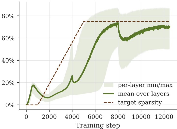
Expected sparsity
