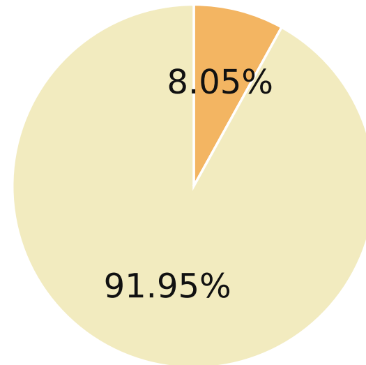
Qwen3-32B-int4-awq
