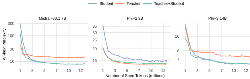
Figure 2.8: The joint loss converges generally better. Convergence of the three losses illustrated in Figure 2.3, evaluated on the Wikitext2 test corpus perplexity during distillation.
