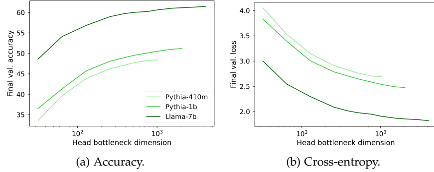
Figure 1.4: Effect of reducing the LM Head rank on accuracy and cross-entropy. Figures from Godey, Clergerie, and Sagot [45].
