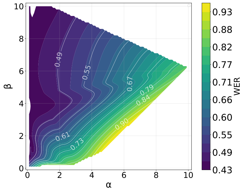
Figure 3.3: Choice of \alpha and \beta . Bayesian hyperparameter search indicates that the main constraint is to keep the lower-layer weight \alpha small.
