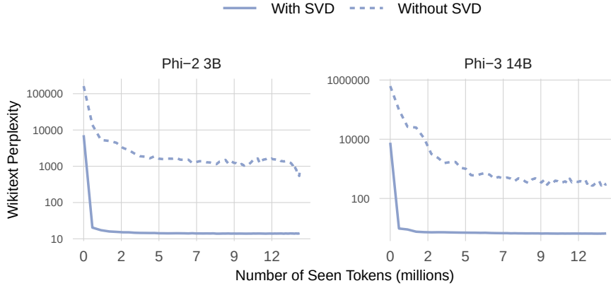
Figure 2.7: SVD Initialization improves the sample-efficiency. Convergence when initializing low-rank weights randomly (without SVD) or with SVD.
