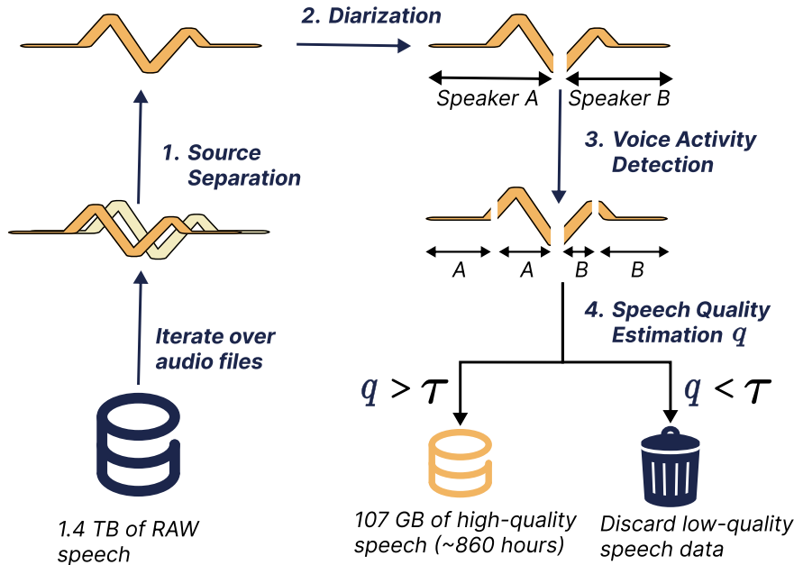
Figure 4.1: Collection of spontaneous Wolof speech for continued self-supervised pretraining. Raw web audio passes through source separation, speaker diarization, voice activity detection, and speech-quality filtering.
