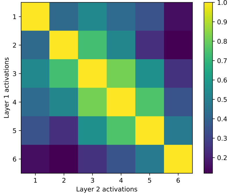
Figure 3.4: Activation similarities between all decoder-layer pairs. Consecutive layers tend to be more similar, suggesting that they can be merged.
