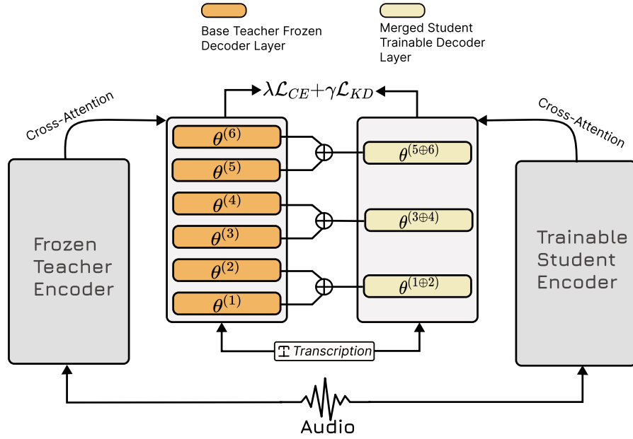
Figure 3.1: Layer merging in the Whisper decoder: each student layer is a weighted average of two consecutive teacher layers, then trained with cross-entropy and knowledge distillation.
