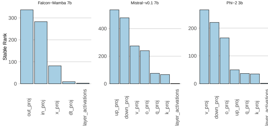
Figure 2.2: Activations are low-rank. Comparison of the stable rank of weights (*_proj) and layer activations (layer_activations). Each bar is the average stable rank across all layers.
