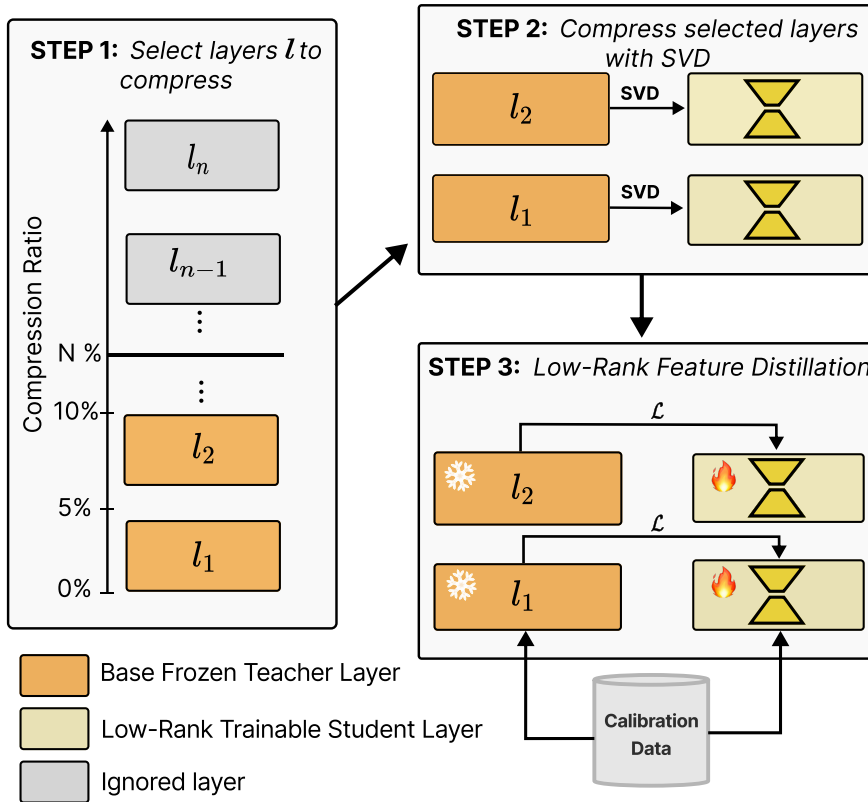
Figure 2.1: Lillama approach : STEP 1 selects layers to compress for a target compression ratio (e.g., N\% ) using various strategies (see Section 2.6). STEP 2 compresses and initializes the chosen parameters via SVD. STEP 3 distills the low-rank weights with a small calibration dataset.
