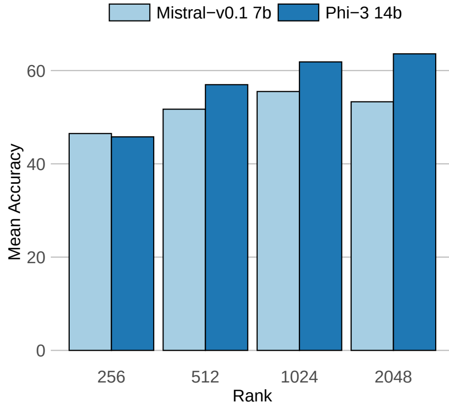
Figure 2.6: Higher ranks give generally better results. Mean accuracy over our test benchmarks as a function of the minimum rank k in Algorithm 1
