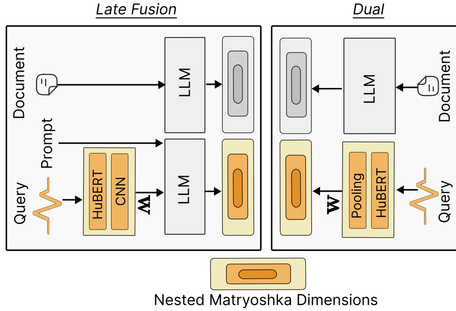
Figure 4.4: Late-fusion and dual architectures. Late fusion projects down-sampled HuBERT features into the LLM embedding space and concatenates them with prompt embeddings. The dual architecture pools speech features and uses dimension-specific projections.
