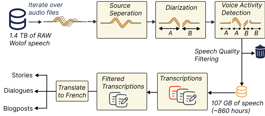
Figure 4.3: Speech data pipeline. Raw data is processed through source separation, diarization, voice activity detection, and quality filtering. Retained speech is transcribed before French stories, dialogues, and blog posts are generated.
