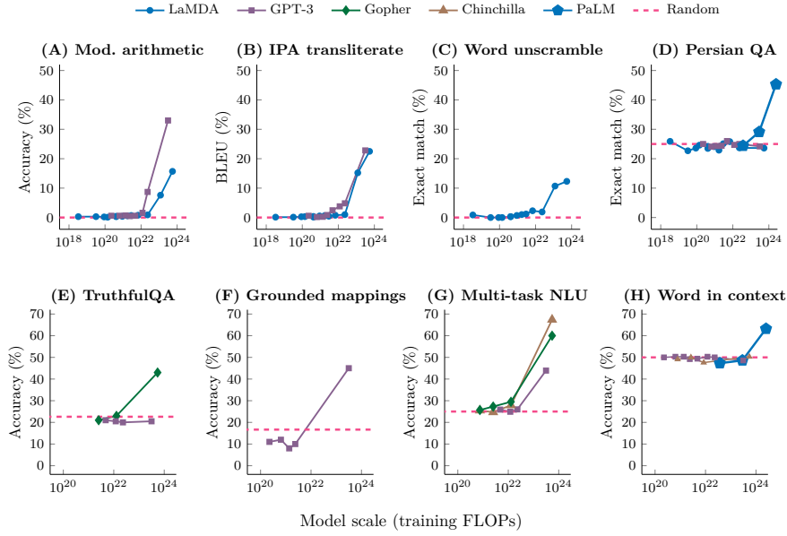
Figure 1.5: Examples of emergent abilities in large language models. Figure from Wei et al. [110]. A capacity is emergent when the score surpasses the random baseline while it wasn't at smaller scale.
