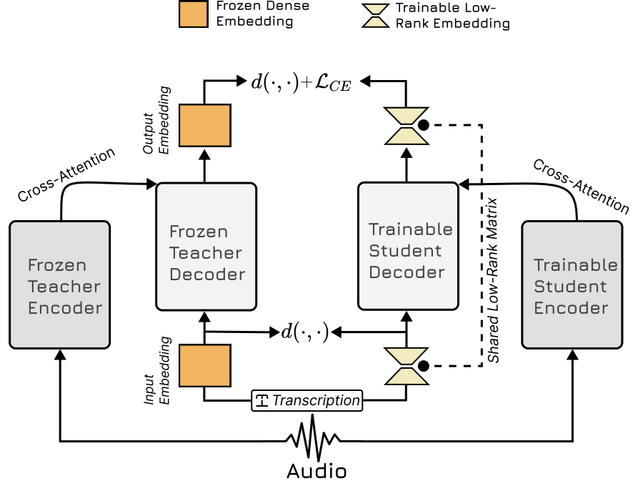
Figure 3.2: Head shearing of the Whisper embedding through low-rank decomposition. The decomposition is activation-aware because the low-rank weights are subsequently feature-distilled.
