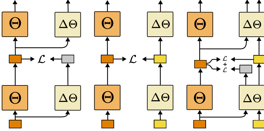
Figure 2.3: Accelerating convergence through a joint loss. We compare three distillation strategies: (a) Teacher, (b) Student, and (c) Teacher+Student.
