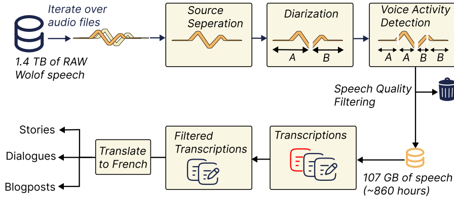
Figure 5.3: Speech data pipeline. Raw data is processed through source separation, diarization, voice activity detection, and quality filtering. Retained speech is transcribed before French stories, dialogues, and blog posts are generated.
