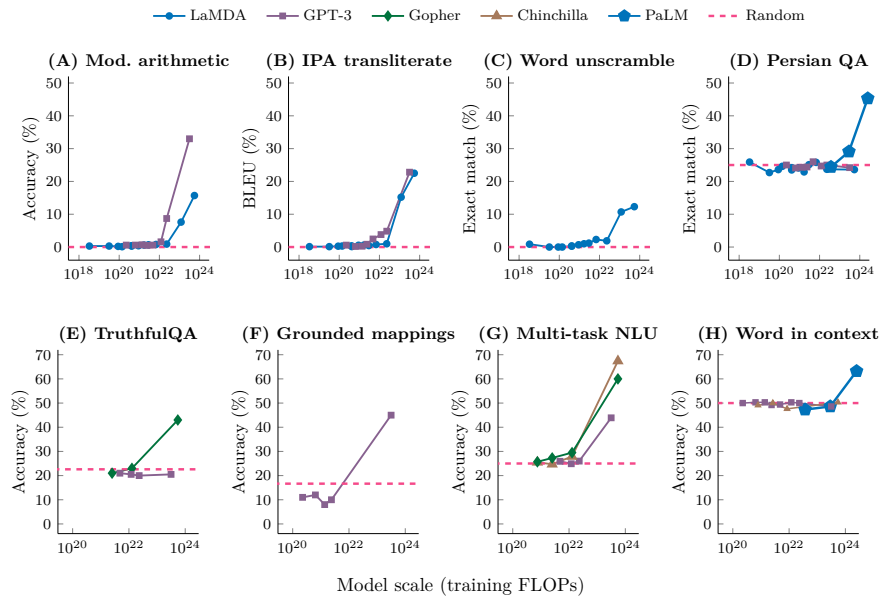
Figure 1.4: Examples of emergent abilities in large language models. Figure from (Wei et al., 2022). A capacity is emergent when the score surpasses the random baseline while it wasn't at smaller scale.
