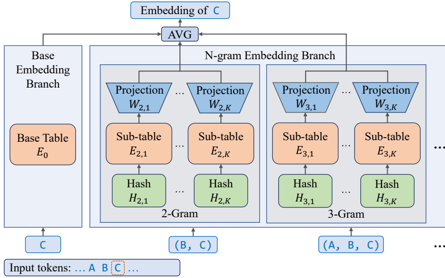
Figure 2.15: Architecture of an n -gram embedding layer. The token embedding is augmented with hashed n -gram embedding branches. Figure from (Liu et al., 2026b).
