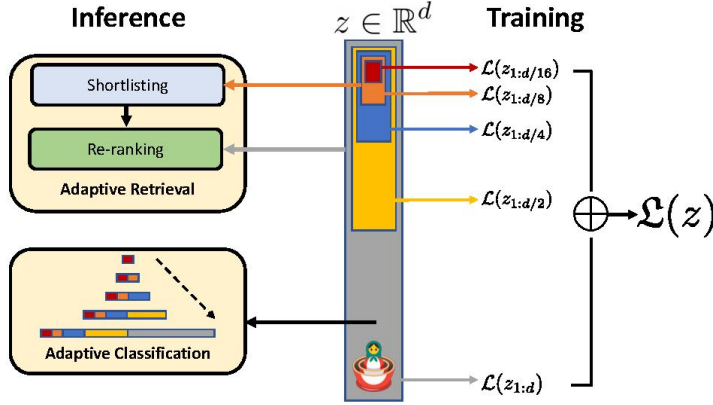
Figure 2.16: Matryoshka Representation Learning trains a representation to be useful at several embedding dimensions. Figure adapted from (Kusupati et al., 2022).
