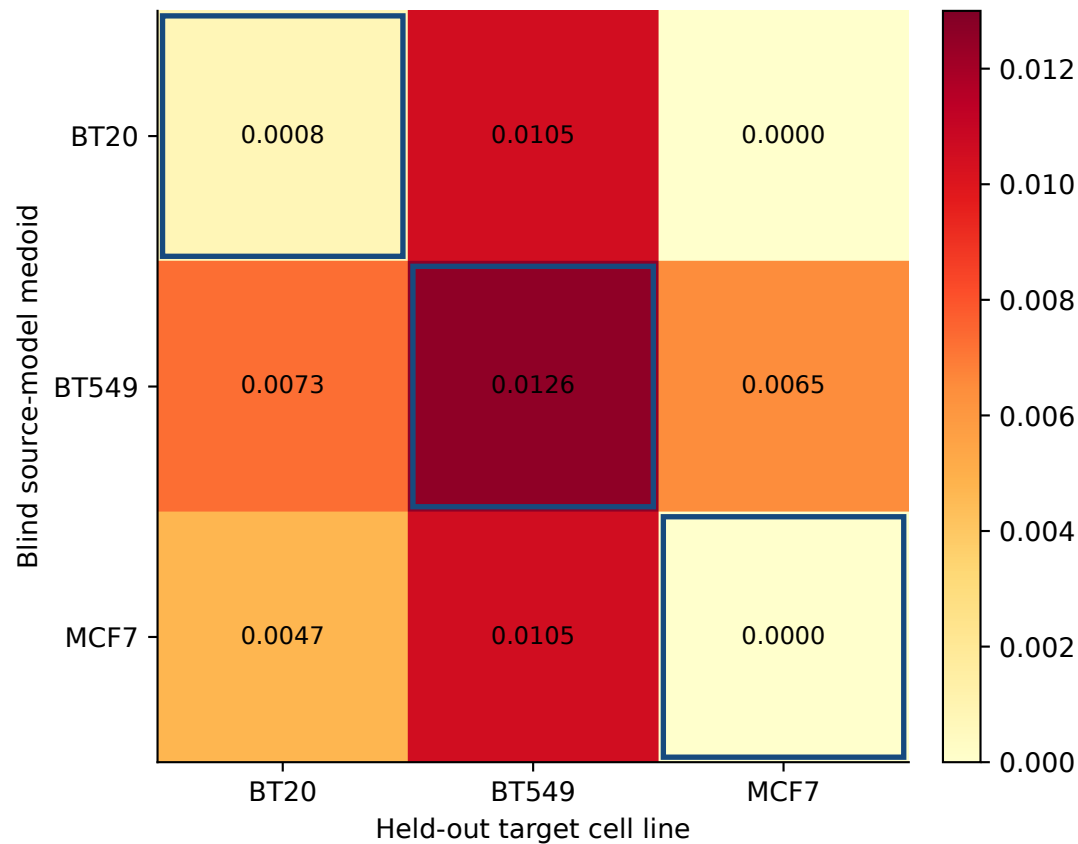
(a) CASPOTS excess RMSE
