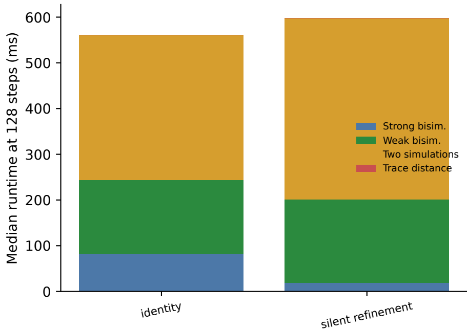
Runtime decomposition
