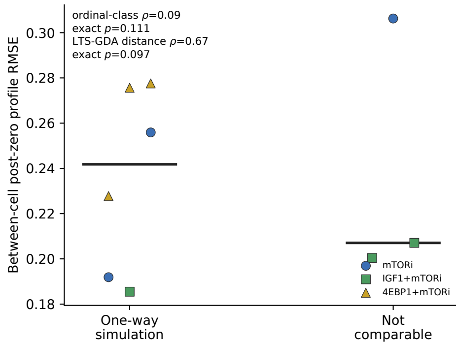
Data distance by formal class
