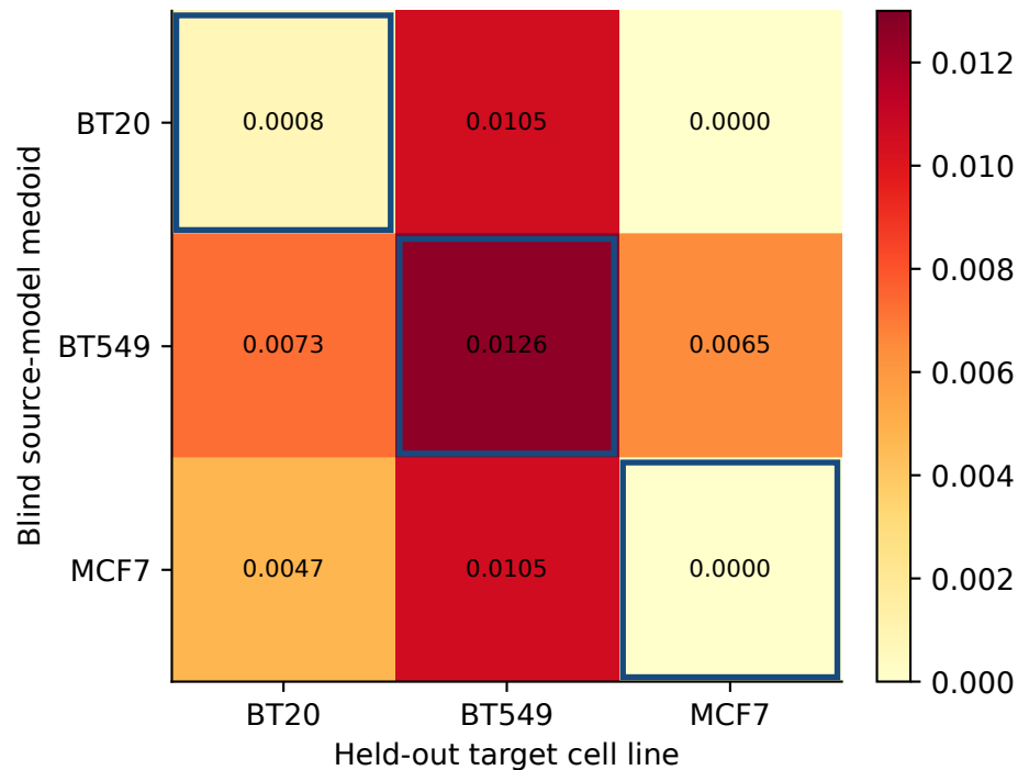
CASPOTS excess RMSE
