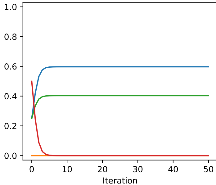
Business C_B
