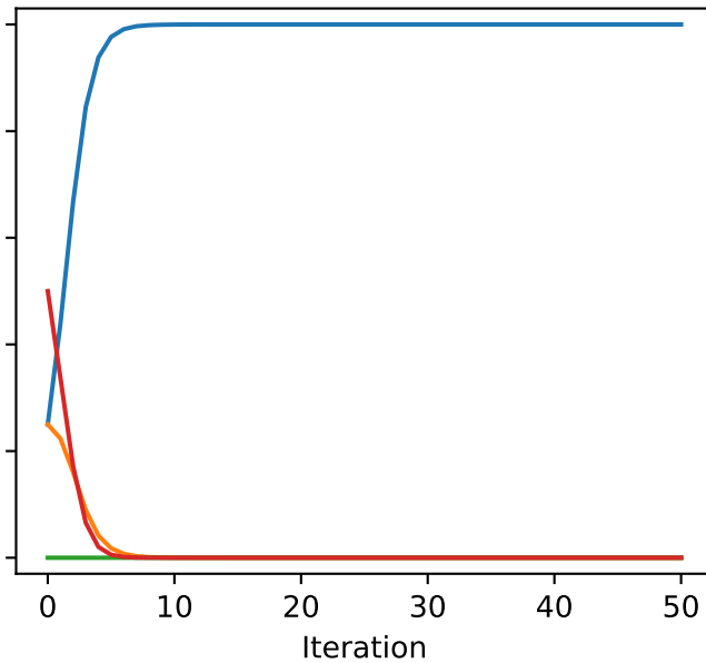
Classroom C_A
