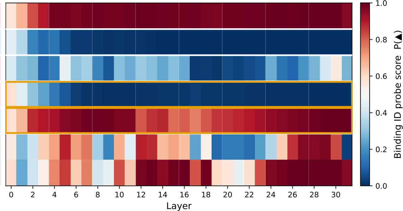
Confused: "Hi Alice!" Model Answer: Thailand
