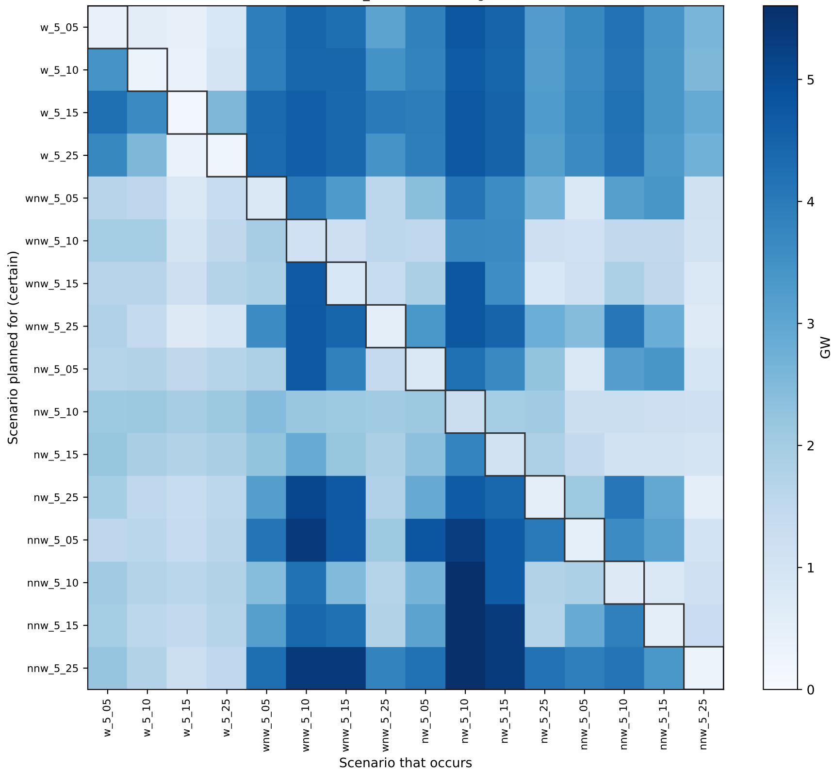
Load shed L(x_k, k') in GW, budget $20M
