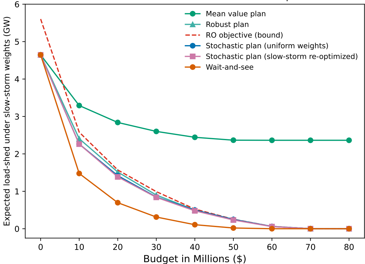
Slow-storm vs Uniform: Stochastic Solution Comparison
