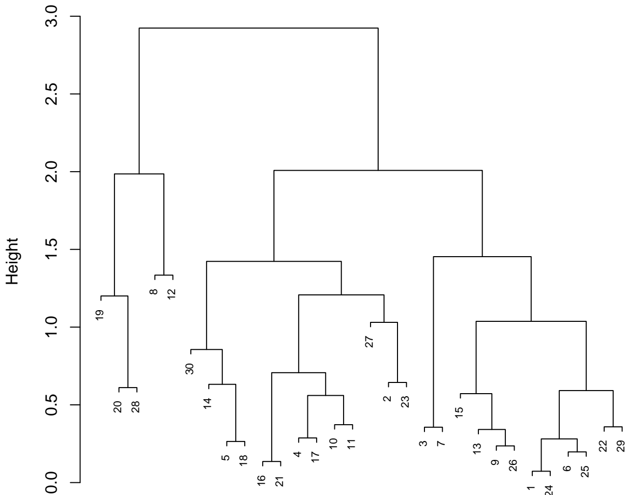
Hierarchical Clustering Dendrogram (average linkage)
