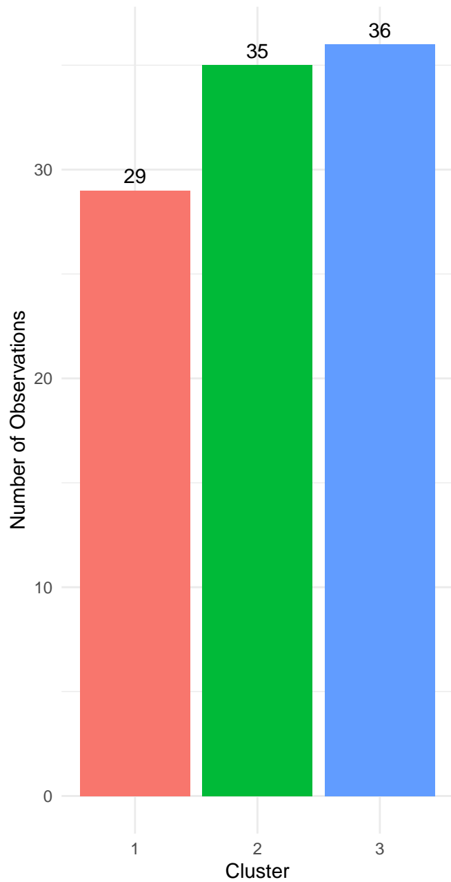
Cluster Size Distribution
