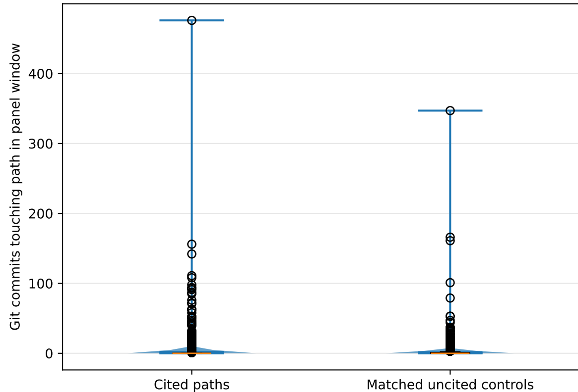
Cited vs uncited path churn contrast
