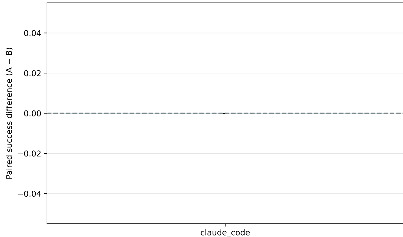
RQ5 causal evidence — effect sizes
