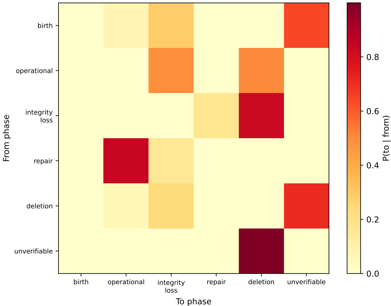
RQ4 — Lifecycle transition probability matrix
