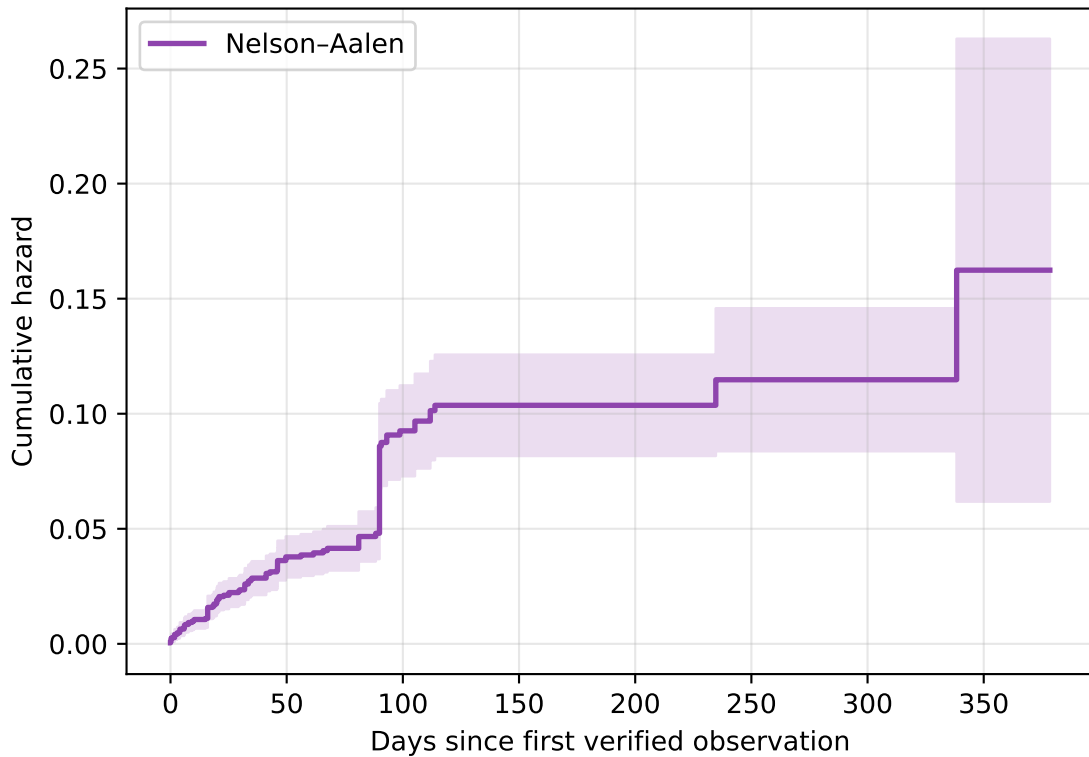
RQ2 — Cumulative hazard of reference failure
