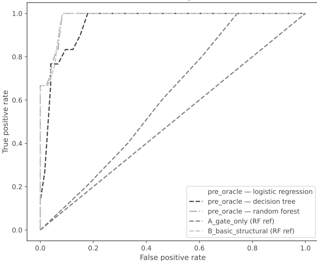
Pre-oracle ROC (out-of-fold) vs gate/structural baselines
