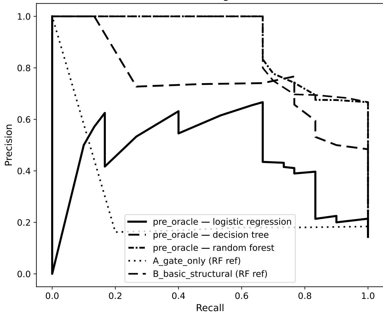
Pre-oracle PR (out-of-fold) vs gate/structural baselines
