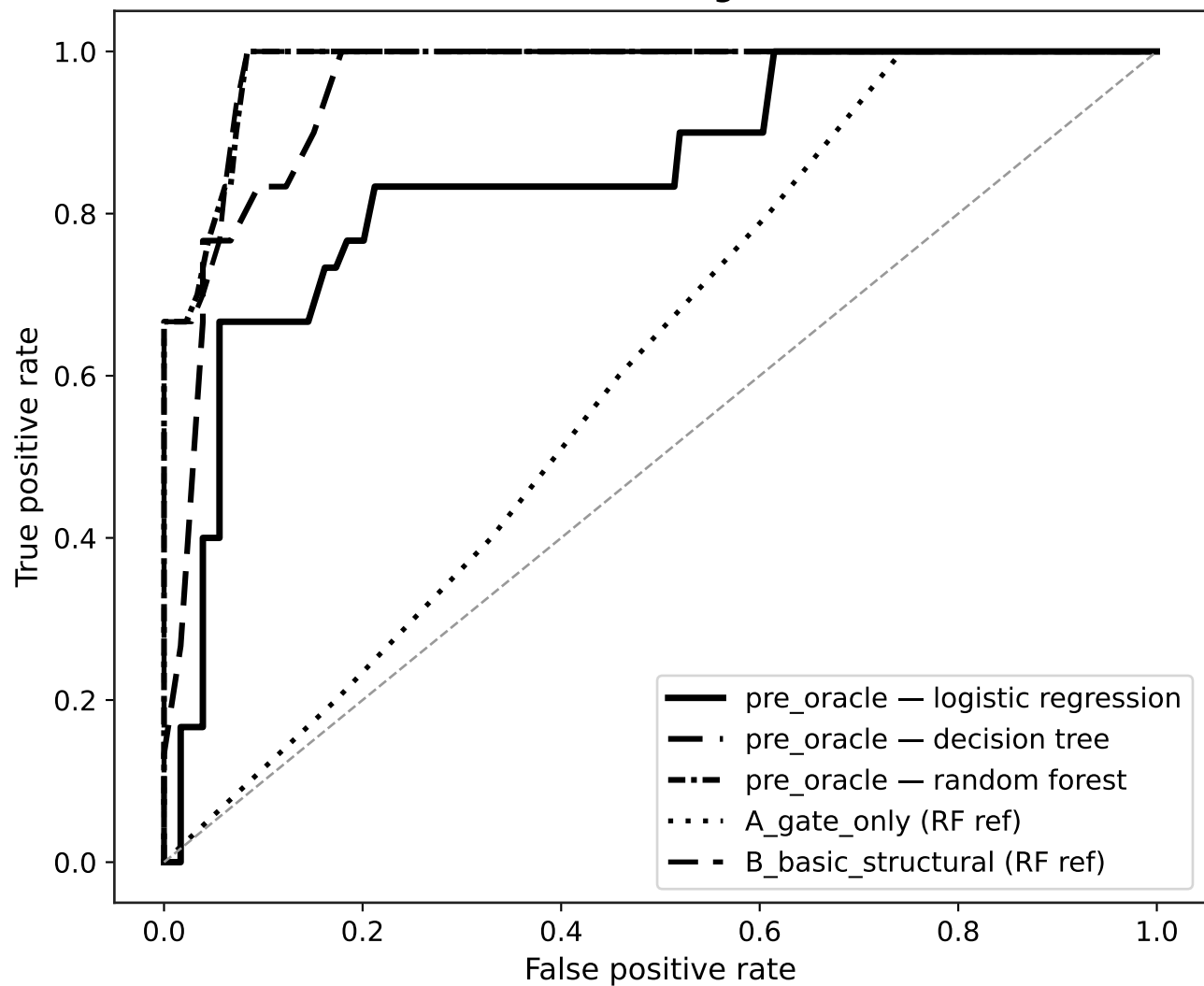
Pre-oracle ROC (out-of-fold) vs gate/structural baselines
