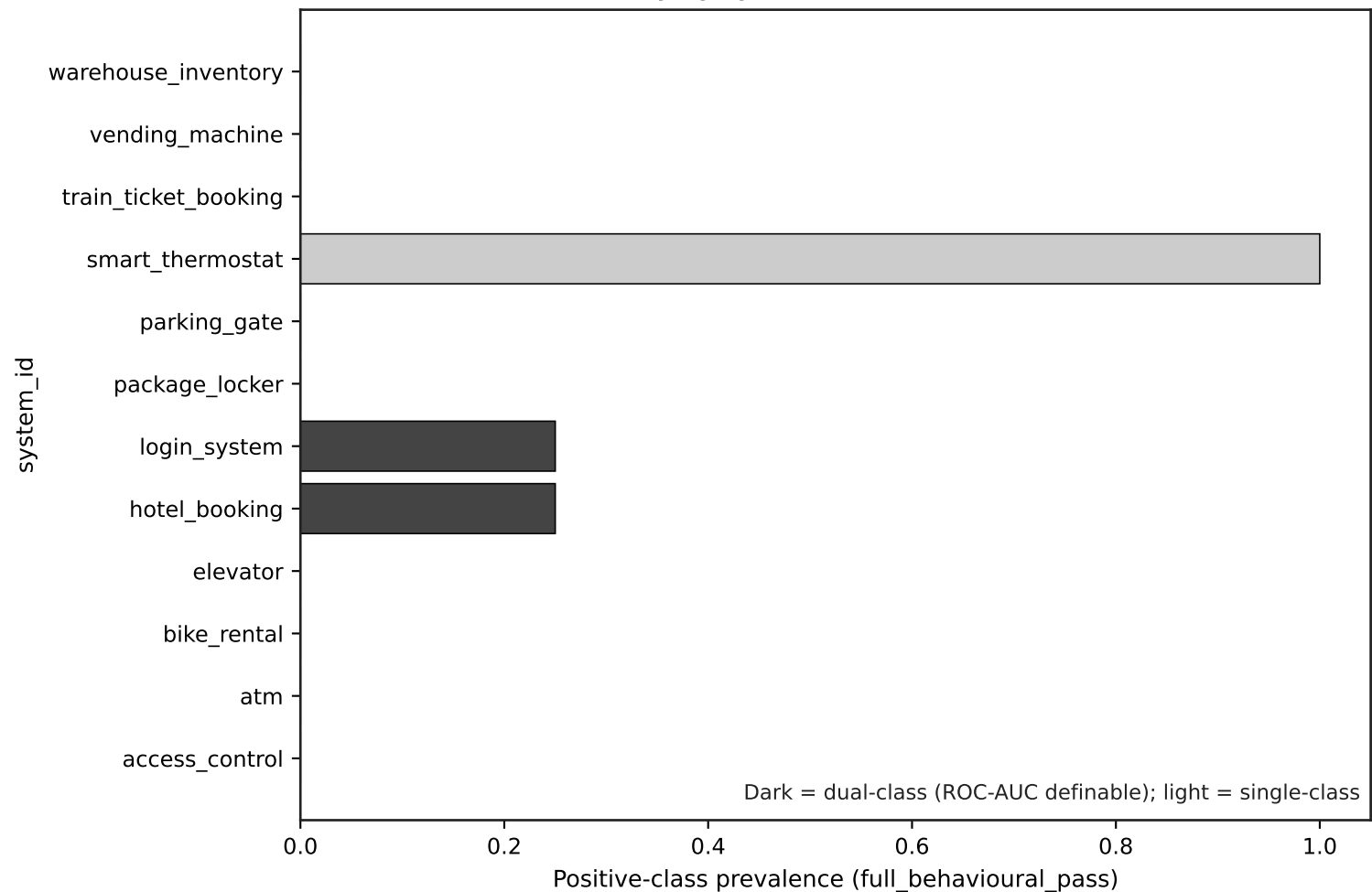
LOSO ROC-AUC definability by system
