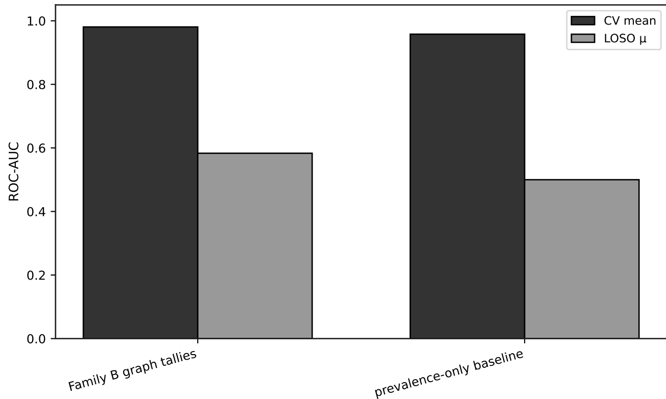
Family B vs prevalence-only baseline
