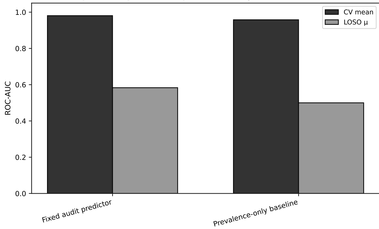
RAP-AQ Step 3: audit predictor vs prevalence-only baseline
