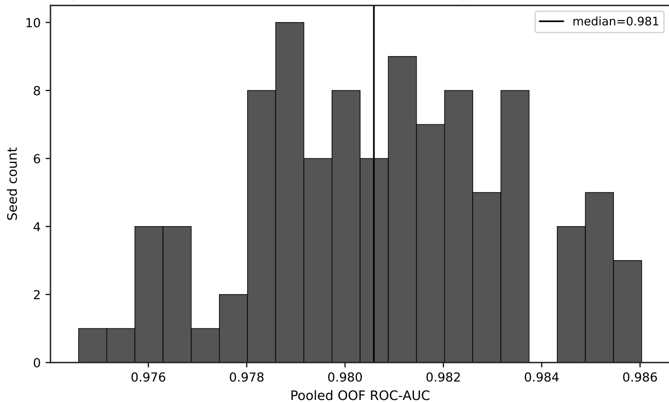
Repeated-seed CV ROC-AUC distribution (fixed audit predictor contract)
